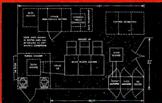
A typical floor layout for the BTF-50A. Additional equipment units provided with the transmitter, but not mounted within the units are: pre-emphasis network, harmonic attenuation, transmission-line monitor, and a console which provides for audio and transmitter control. Write to nearest RCA sales office for details on various suggested floor plan arrangements.
